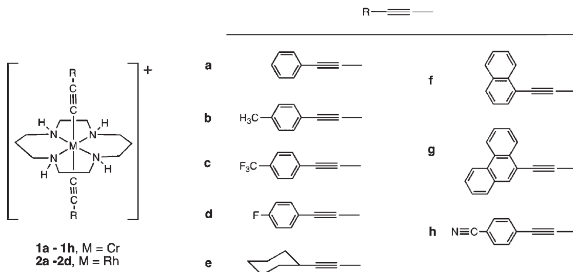
Figure 1. [M(\text{cyclam})(\text{CCR})_2]\text{OTf} complexes discussed in this paper. The abbreviations 1a–1h and 2a–2d are used to refer to the trans complexes. The cis complexes will be referred to as cis-1a–1h .
