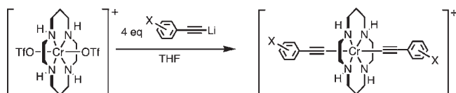
Figure 3. General synthetic scheme for 1a–1c .
