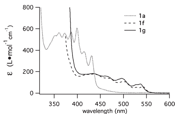
Figure 7. UV-vis absorption spectra (in \text{CH}_3\text{CN} ) comparing 1a with 1f and 1g . Note that the expanded aromaticity shifts the onset of absorption to longer wavelengths.
