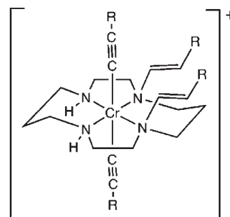
Figure 4. Structure of the product resulting from hydroamination.
