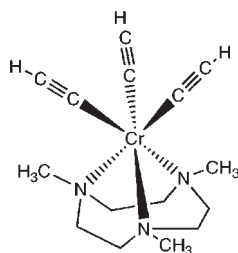
Figure 2. (\text{Me}_3\text{tacn})\text{Cr}(\text{CCH})_3 .
