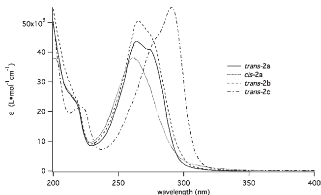
Figure 8. UV–vis absorption spectra of Rh(III) alkynyl complexes in CH 3 CN. The spectrum for trans - 2a was also recorded in THF and water, demonstrating that the spectra are largely solvent independent. The Beer's Law dependence was also demonstrated for trans - 2a in CH 3 CN.
