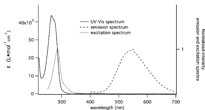
Figure 9. Absorption, emission ( \lambda_{\text{ex}} = 290 nm), and excitation ( \lambda_{\text{em}} = 548 nm) spectra for 2a in degassed acetonitrile.
