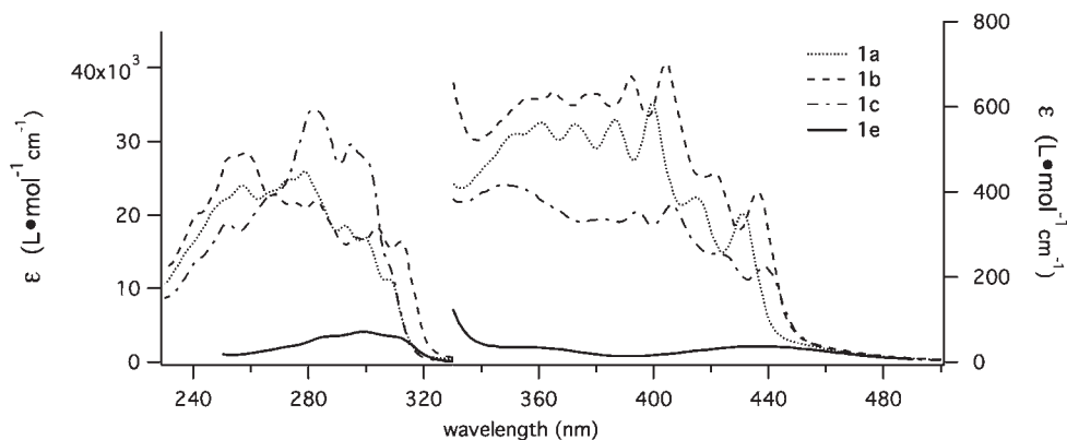
Figure 6. UV-vis absorption spectra (in \text{CH}_3\text{CN} ) comparing selected trans -[Cr(cyclam)(CCR) _2 ]OTf complexes, 1a–1c and 1e .
