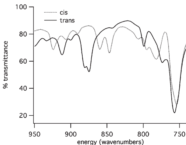
Figure 5. Infrared spectra in the \text{CH}_2 rocking and \text{NH} bending region for the cis and trans isomers of 1a .
